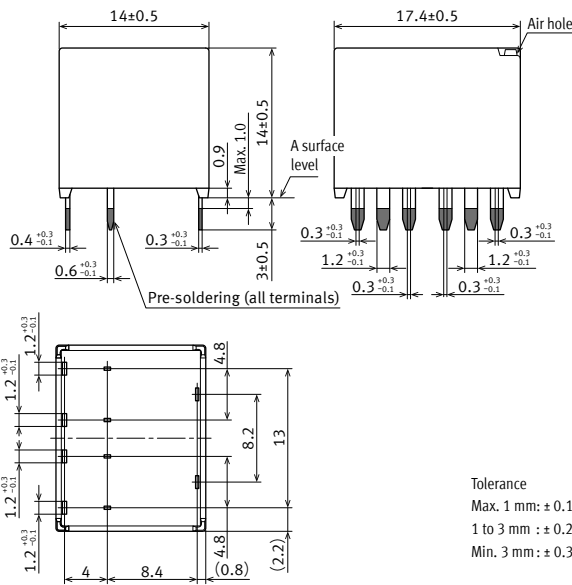
External dimensions
